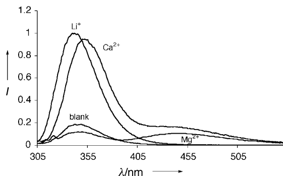
Figure 2. Curves for the titration of 2 ( 1 \times 10^{-5} M in CH 3 CN) with alkaline and alkaline earth cations.
